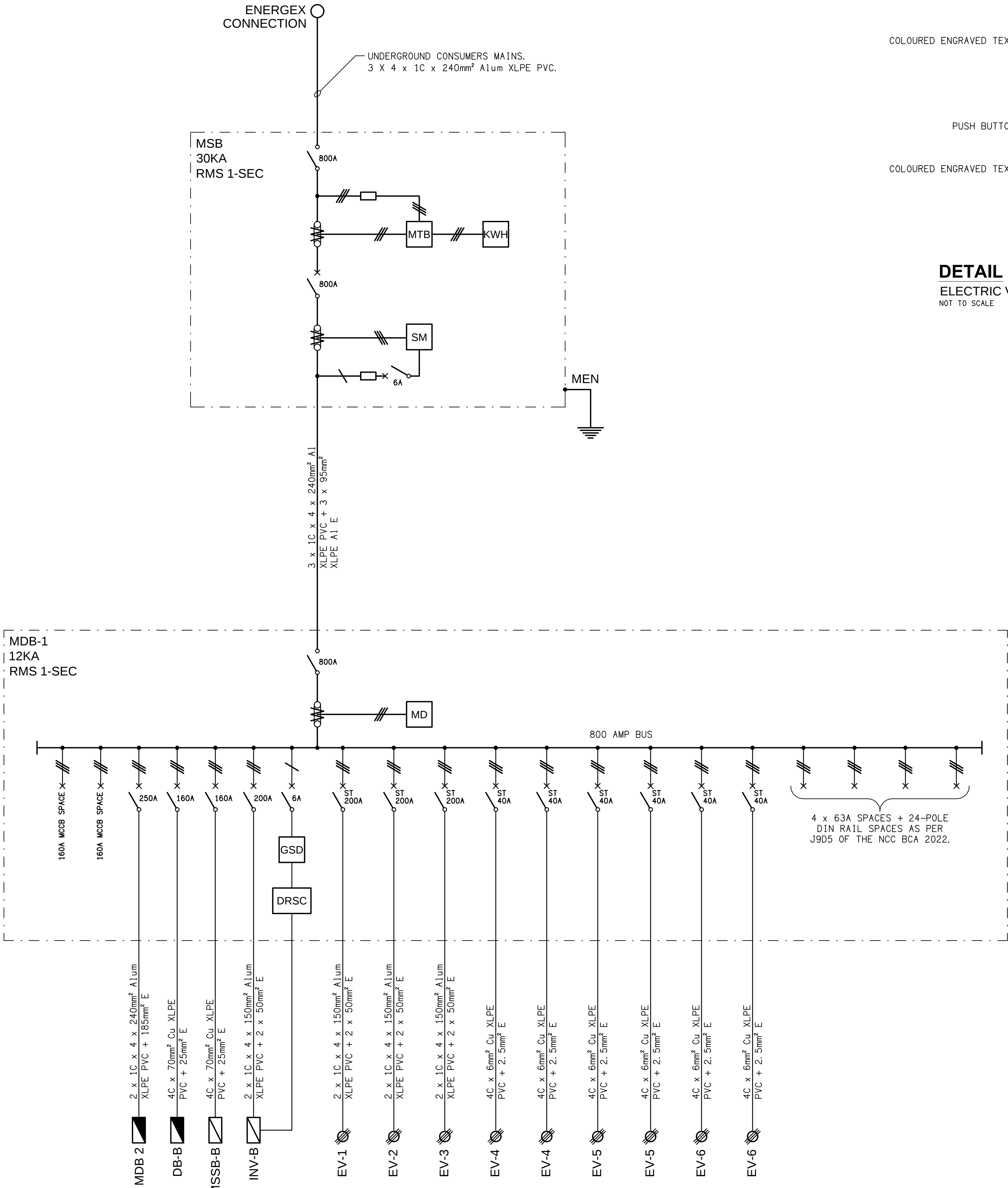
SCHEMATIC MSB-B CONFIGURATION NOT TO SCALE
